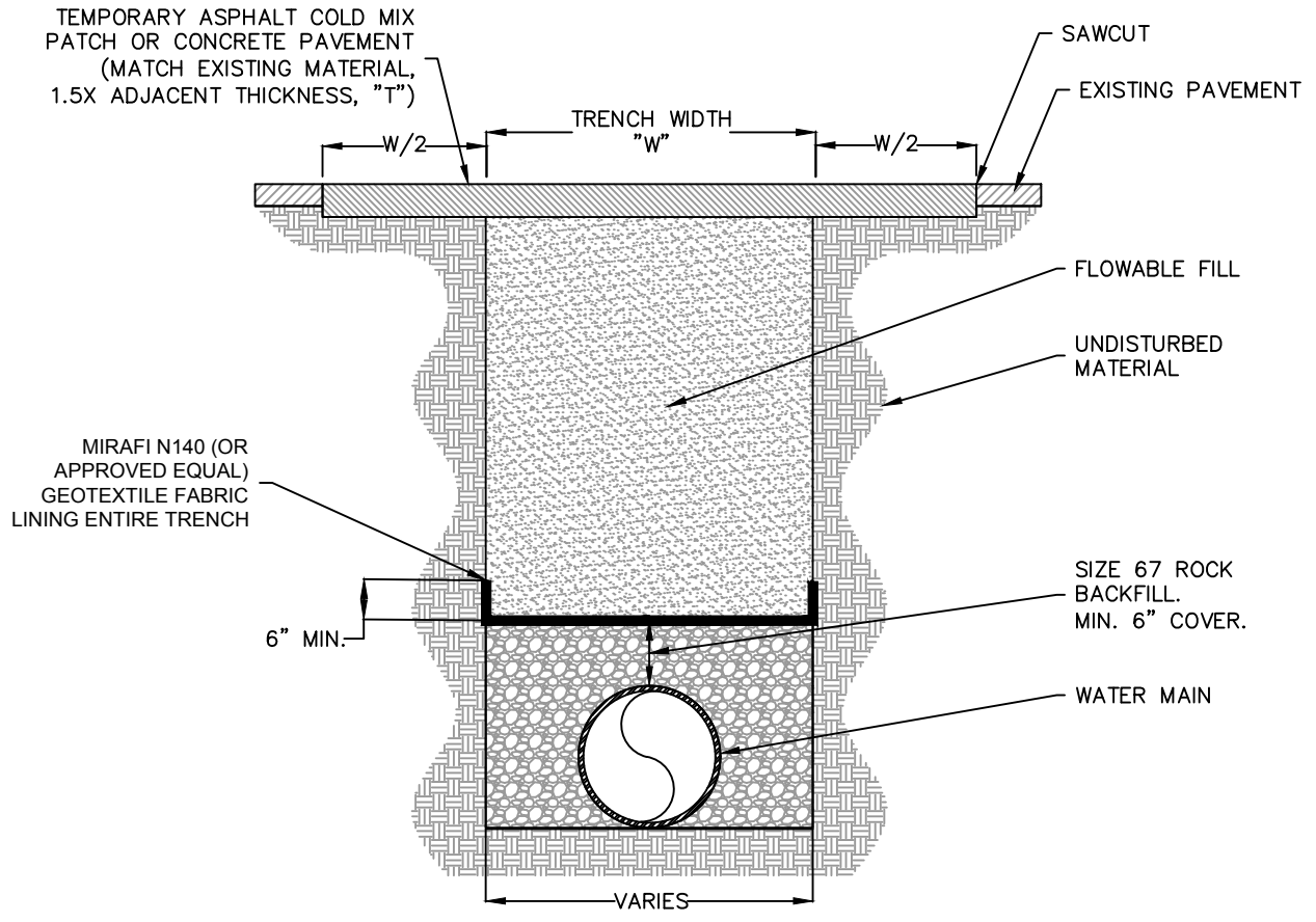
PROFILE VIEW
