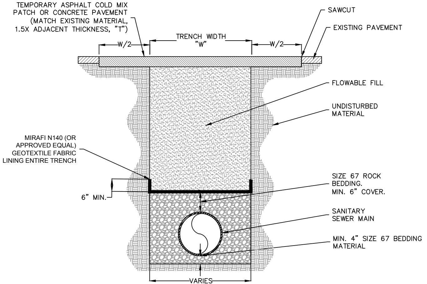
PROFILE VIEW
