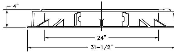
FRAME SECTION
