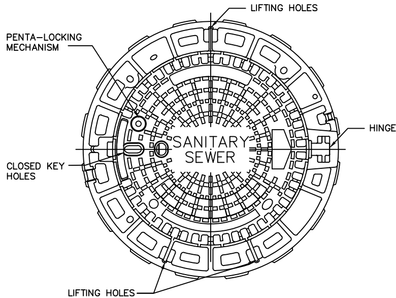
MANHOLE DETAIL
