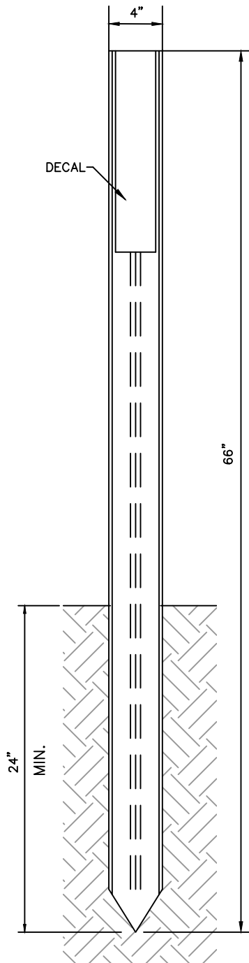
FIBERGLASS POST STOCK NO: RHIND 3-RAIL
