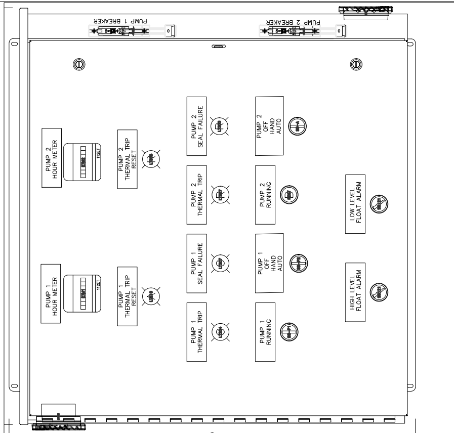
PUMP CONTROL PANEL FRONT PANEL LAYOUT
