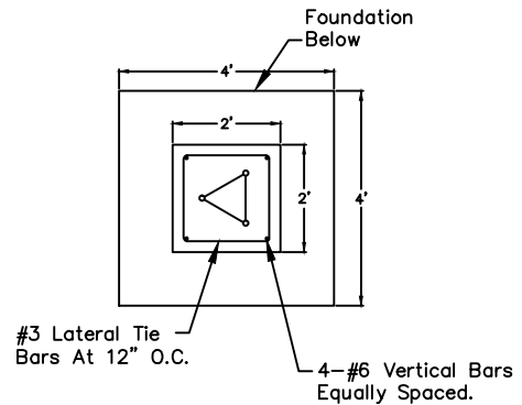
TOWER SECTION
