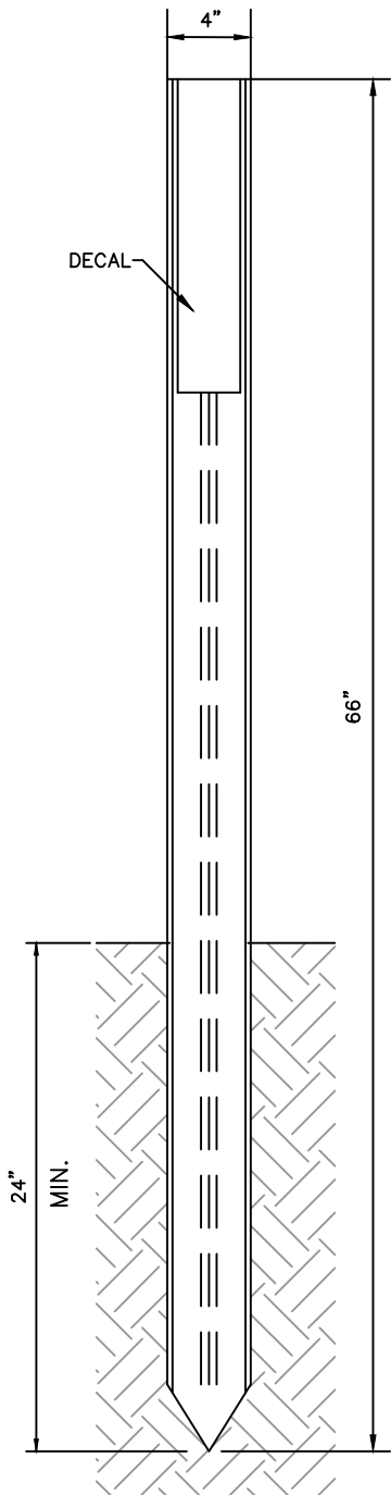
FIBERGLASS POST STOCK NO: RHIND 3-RAIL
