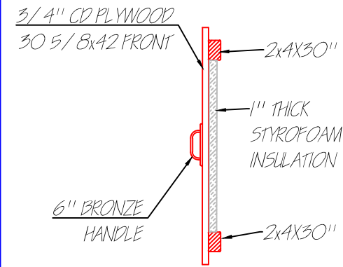
PLAN VIEW (REMOVABLE LIFT-OUT END SECTION)
