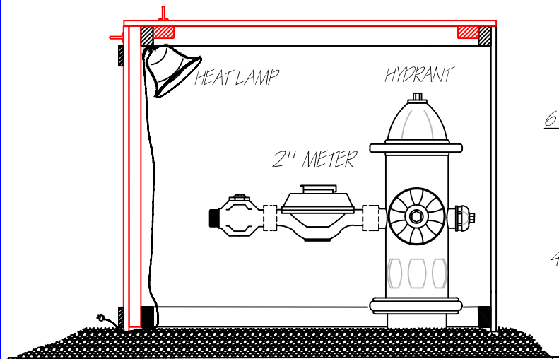
SECTION THRU BOX (WITHOUT INSULATION)
