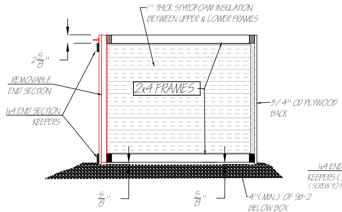
SECTION A-A (WITHOUT TOP LID)
