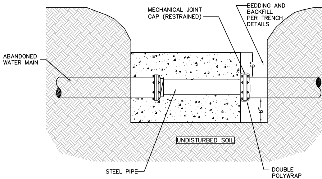
PROFILE VIEW
