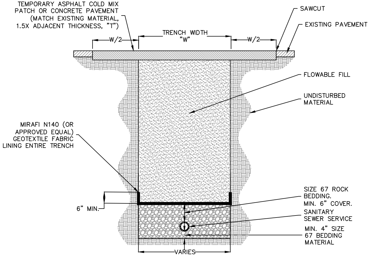
PROFILE VIEW SECTION A-A
