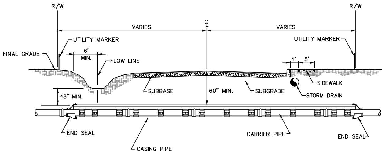
TYPICAL HIGHWAY BORING (SEWER LINE SHOWN...WATER LINE SIMILAR) N.T.S.
