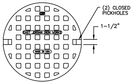
MANHOLE COVER
