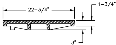
COVER SECTION
