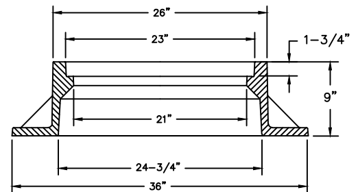
FRAME SECTION
