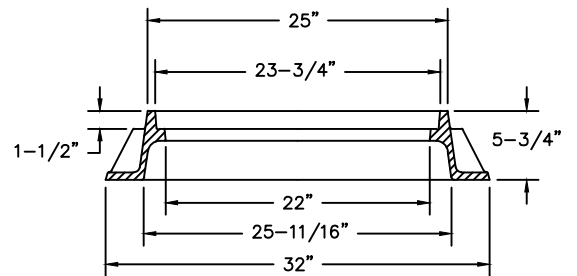
FRAME SECTION
