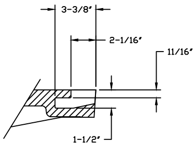
PICKHOLE DETAIL
