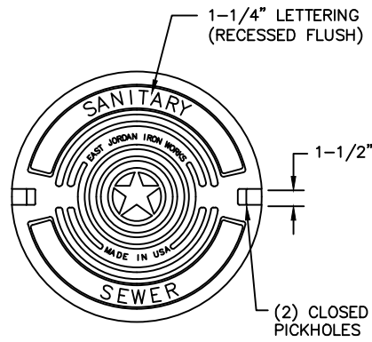
MANHOLE COVER
